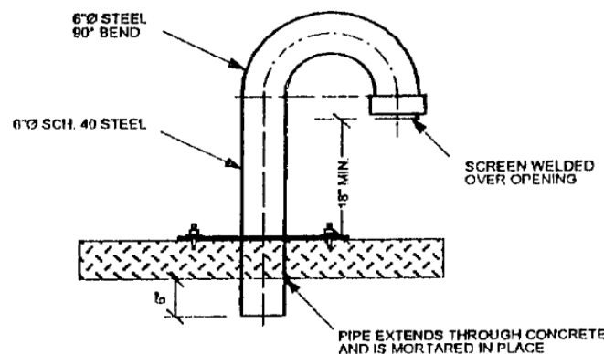
VENT PIPE DETAIL SCALE 1:25
