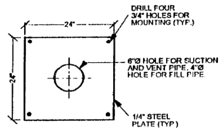
SUCTION, FILL AND VENT PIPES SCALE 1:25
