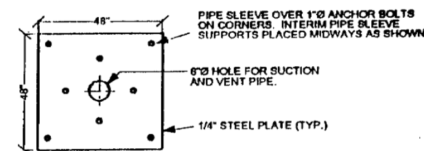
ANTI-VORTEX PLATE PLAN SCALE 1:50
